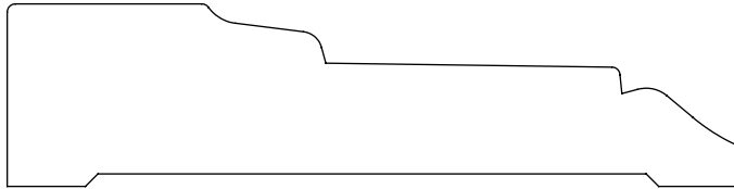
0.875" x 3.500" #2426 Casing
