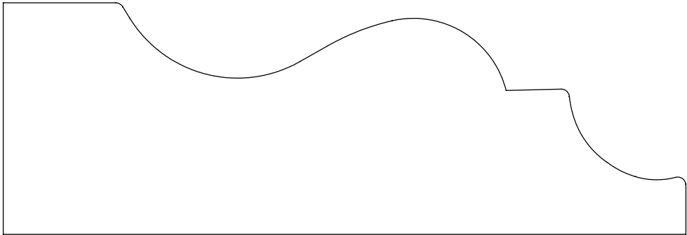
1.750" x 5.160" #4227 Crown
