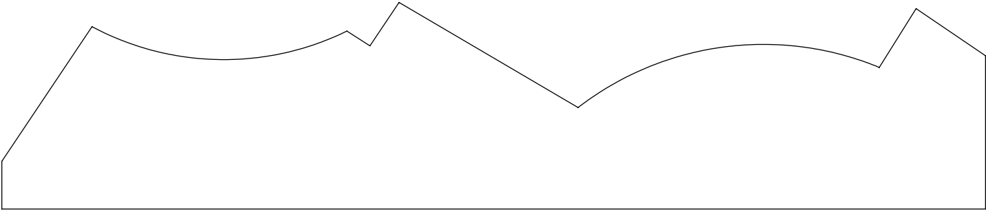
1.563" x 7.437" #4050 Crown
