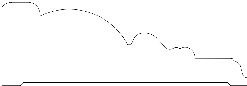
1.687" x 5.000" #2803 Casing
