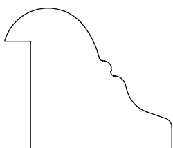
1.062" x 1.250" #5063 Panel Mold
