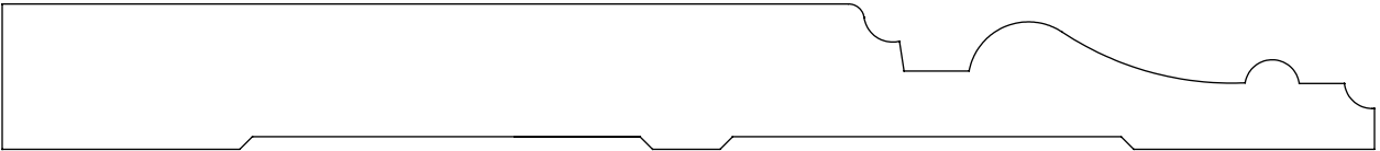
0.687" x 6.500" #1202 Base
