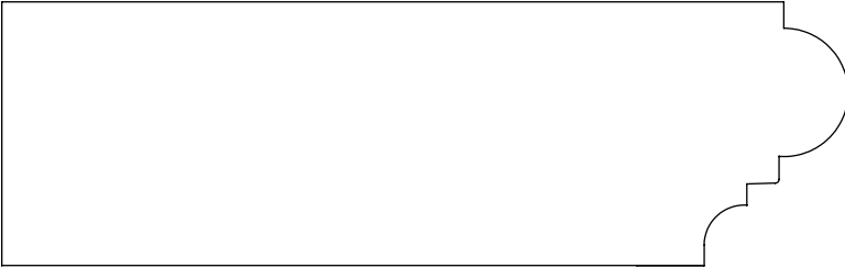
1.250" x 4.000" #6504 Nosing
