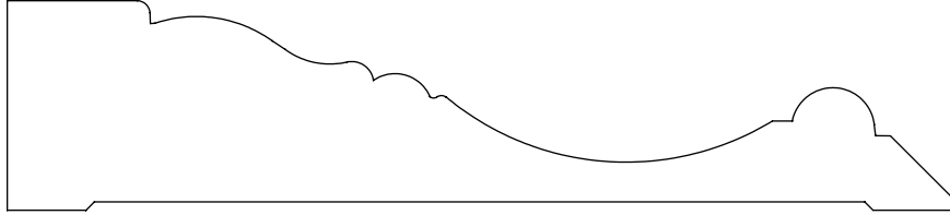
1.000" x 4.500" #2812 Casing
