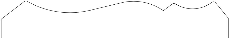
0.750" x 4.562" #4232 Crown
