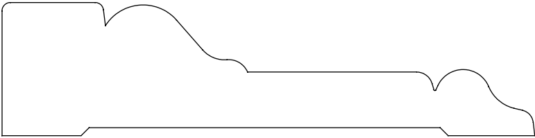
1.000" x 4.000" #2421 Casing
