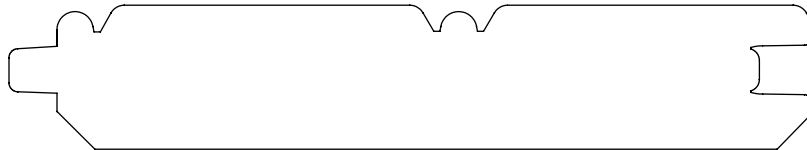
0.750" x 4.182" #8811 Beaded Paneling
