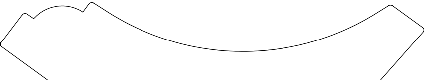
0.812" x 4.420" #4107 Crown
