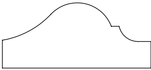
0.687" x 1.562" #5032 Panel Mold
