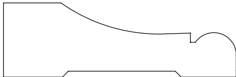
0.750" x 2.375" #2200 Casing
