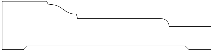
0.812" x 3.500" #2156 Casing
