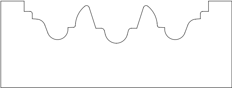
1.500" x 4.000" #2599 Casing
