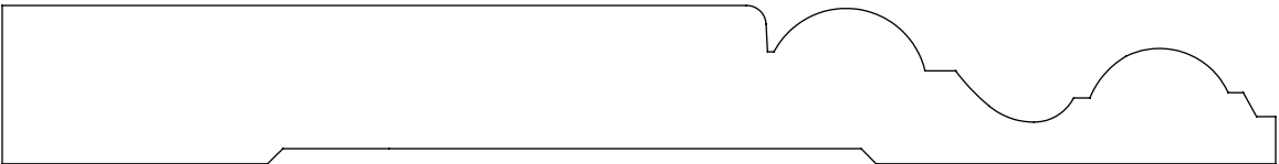
0.750" x 6.000" #1200 Base
