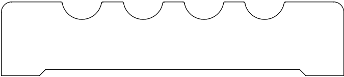
0.750" x 3.500" #2501 Casing
