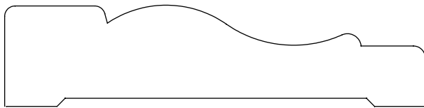
0.750" x 3.125" #2102 Casing
