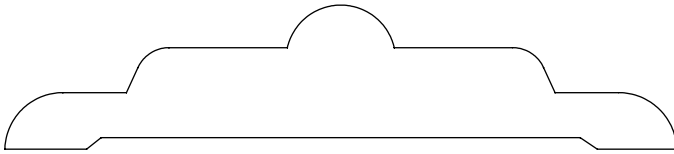
0.750" x 3.500" #2560 Casing
