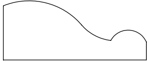
0.625" x 1.510" #5225 Base Cap
