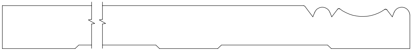
0.750" x 7.500" #1501 Base
