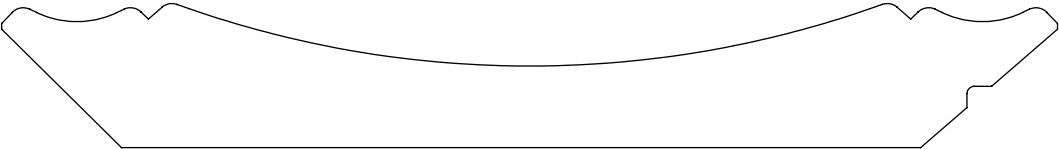
0.750" x 5.500" #4108 Crown
