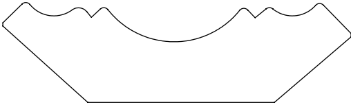
0.750" x 2.625" #4106 Crown
