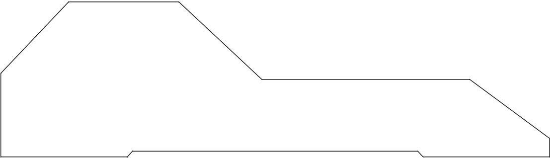
1.625" x 5.750" #2912 Casing
