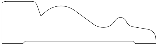
0.750" x 2.750" #2107 Casing
