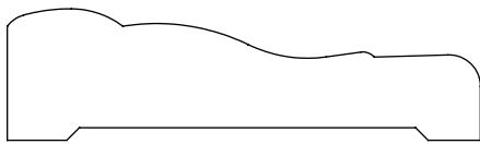
0.625" x 2.250" #2103 Casing
