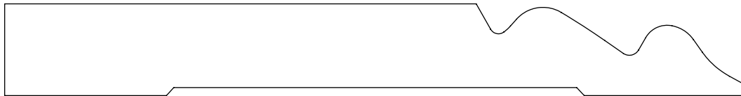
0.687" x 5.500" #1218 Base
