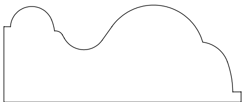
1.000" x 2.437" #8002 Chair Rail
