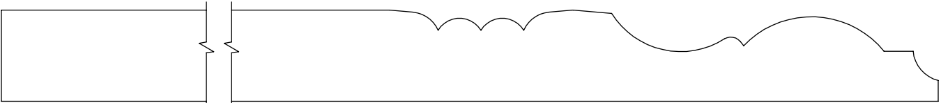
0.687" x 7.500" #1203 Base
