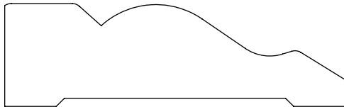
0.750" x 2.500" #2108 Casing
