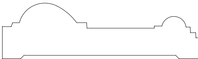
1.000" x 3.500" #8022 Chair Rail
