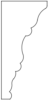
0.812" x 1.750" #4900 Crown
