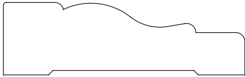
0.750" x 2.500" #2101 Casing
