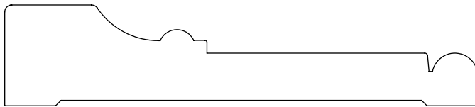
0.750" x 3.480" #2403 Casing
