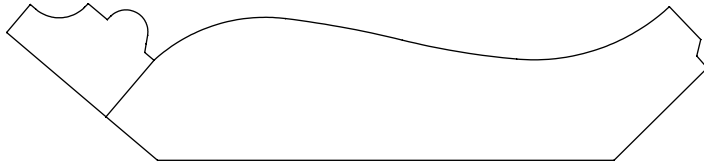
0.812" x 3.650" #4501 Crown
