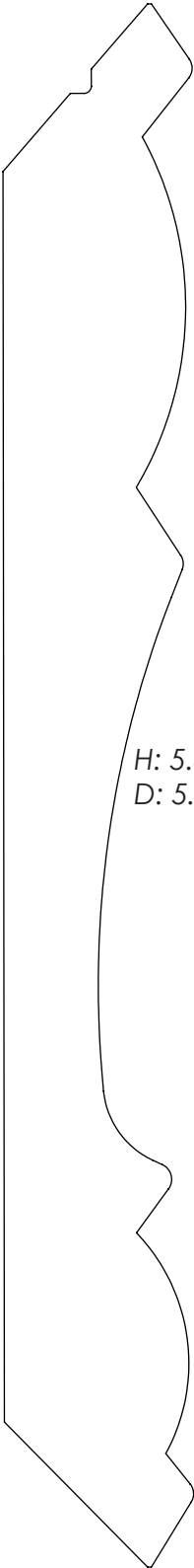
1.000" x 8.250" #4819 Crown
