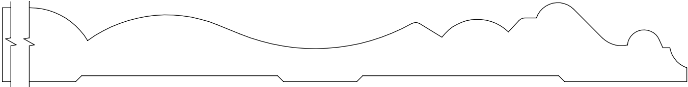
0.812" x 7.500" #1904 Base
