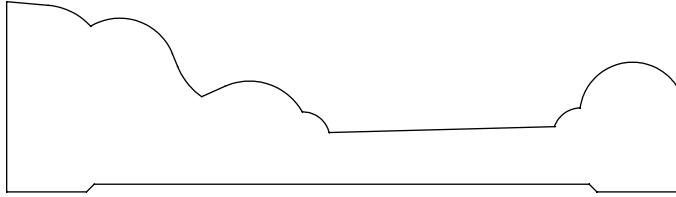
1.000" x 3.500" #2482 Casing
