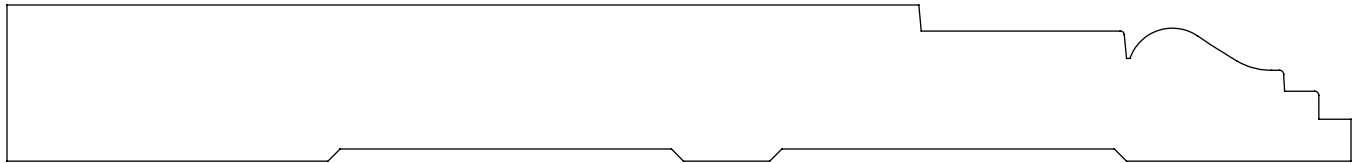
0.812" x 7.000" #1206 Base
