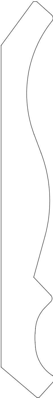
0.937" x 7.187" #4222 Crown
