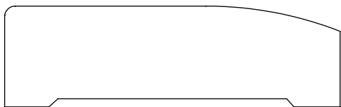
0.750" x 2.500" #2004 Casing
