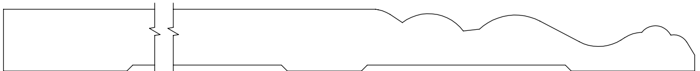
0.625" x 7.500" #1909 Base
