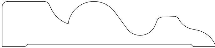
0.750" x 3.563" #2807 Casing
