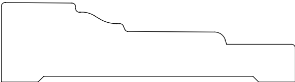
0.812" x 3.000" #2164 Casing
