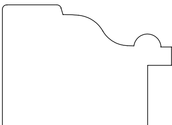
1.250" x 1.750" #3973 Backband
