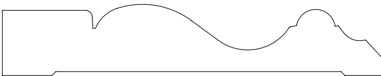
0.750" x 4.000" #2263 Casing
