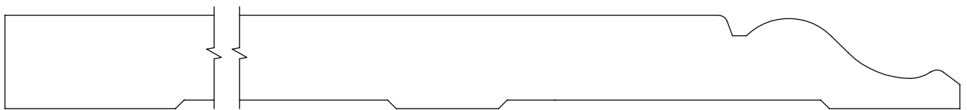
0.687" x 7.500" #1208 Base
