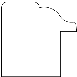
1.250" x 1.250" #3965 Backband
