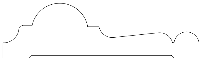
1.000" x 3.500" #8025 Chair Rail
