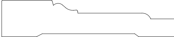
0.750" x 3.535" #2157 Casing
