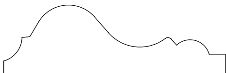
0.750" x 2.375" #8003 Chair Rail
