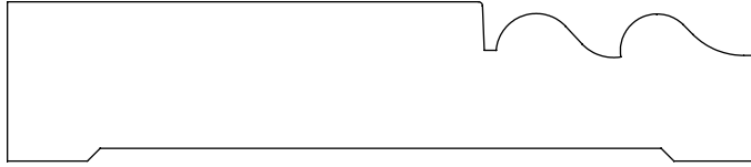
0.750" x 3.500" #2661 Casing
