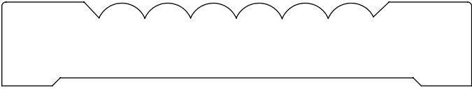
0.625" x 3.500" #2520 Casing
