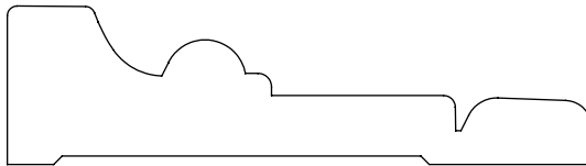
0.750" x 2.770" #2401 Casing
