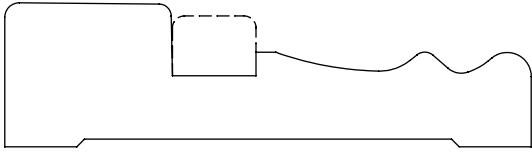
0.750" x 2.750" #2902 Casing
