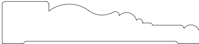
0.750" x 3.490" #2240 Casing
