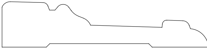
0.780" x 3.545" #2484 Casing
