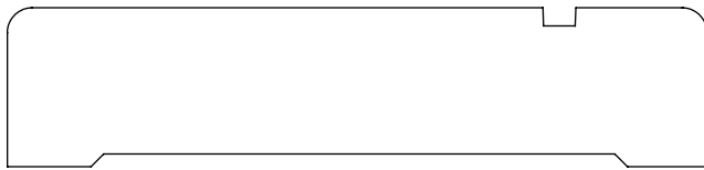
0.750" x 3.290" #2681 Casing
