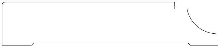
0.750" x 3.750" #2621 Casing
