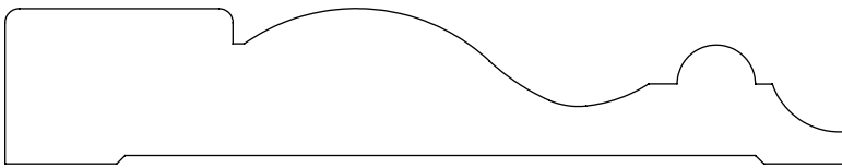
0.750" x 4.000" #2262 Casing
