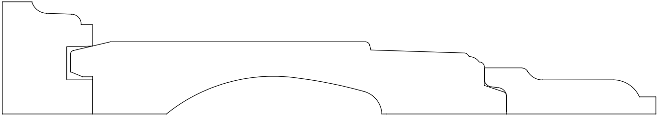
1.250" x 7.286" #1900-1901-5019 Base (shown at 95%)
