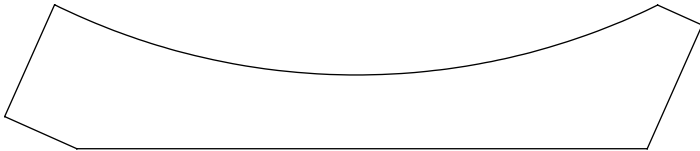
0.750" x 3.625" #4003 Crown
