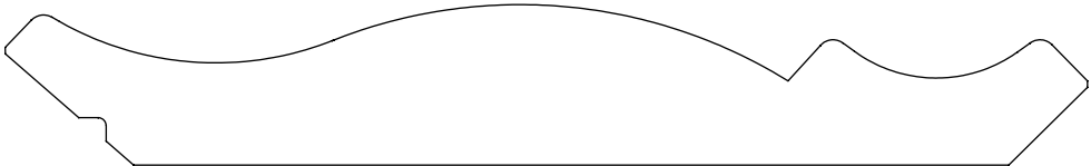
0.750" x 5.062" #4233 Crown
