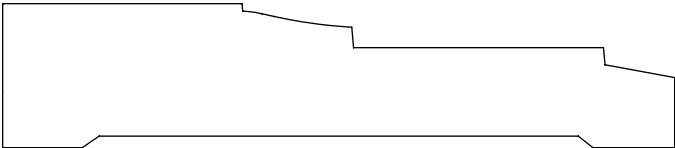
0.750" x 3.500" #2165 Casing
