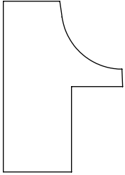
1.250" x 0.875" #3970 Backband
