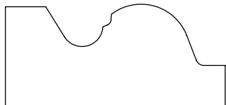
0.750" x 1.625" #5038 Panel Mold
