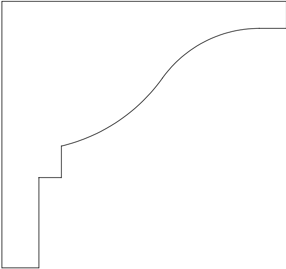
2.937" x 2.750" #4224 Crown
