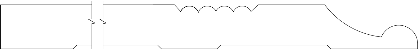
0.750" x 7.500" #1204 Base
