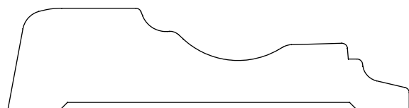
0.750" x 2.945" #8040 Chair Rail
