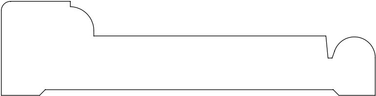
1.000" x 3.990" #2441 Casing
