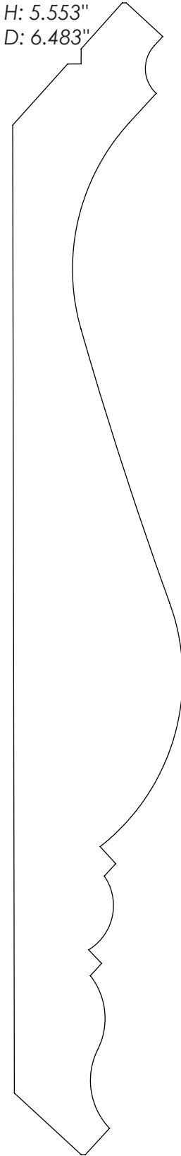
1.250" x 8.500" #4223 Crown
