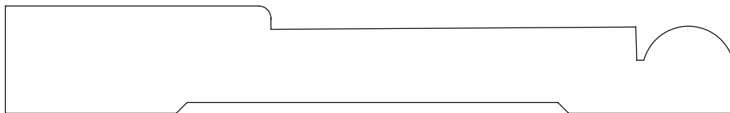
0.812" x 5.500" #1602 Base
