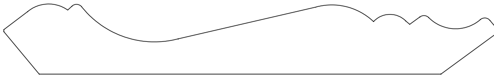
0.750" x 5.250" #4217 Crown
