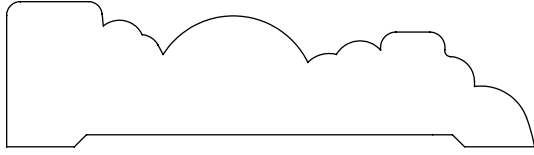
0.750" x 2.750" #2800 Casing
