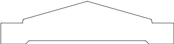
0.750" x 3.000" #2554 Casing
