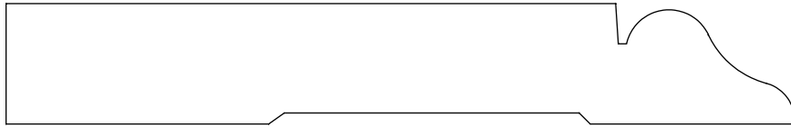
0.687" x 4.500" #1644 Base
