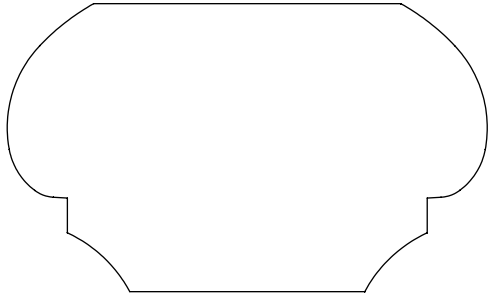
1.500" x 2.500" #6013 Hand Rail
