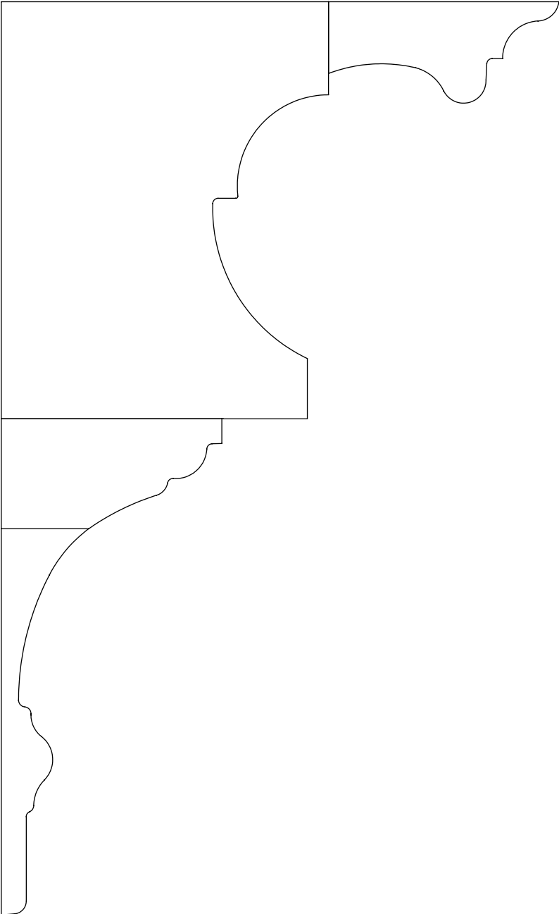
6.750" x 4.125" #4500 Crown
