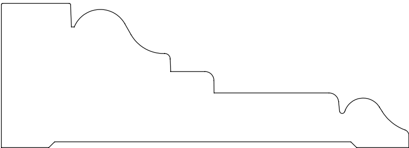
1.500" x 4.230" #2423 Casing
