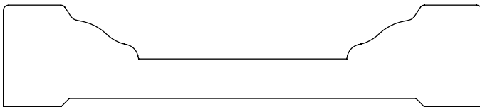
0.750" x 3.500" #2562 Casing
