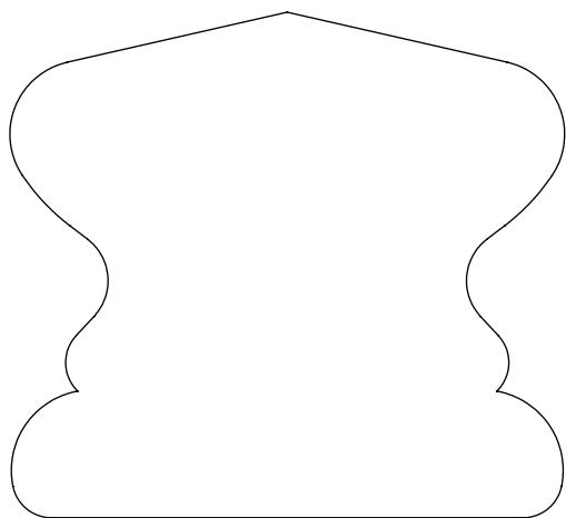
2.368" x 2.598" #6022 Hand Rail
