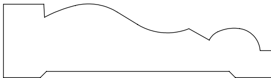
0.750" x 2.750" #2815 Casing
