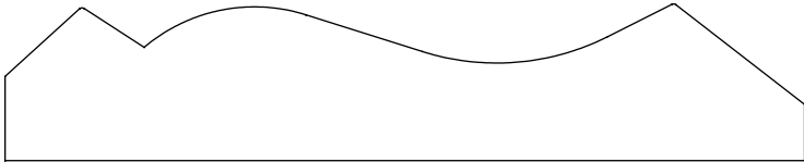
0.750" x 3.812" #4208 Crown
