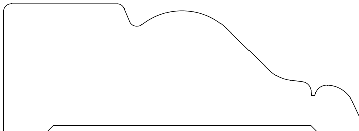
1.312" x 3.656" #2428 Casing
