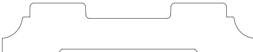
0.875" x 4.500" #8506 Chair Rail
