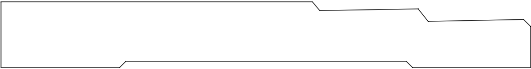
0.687" x 5.500" #1040 Base
