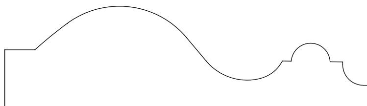
1.062" x 3.875" #8014 Chair Rail
