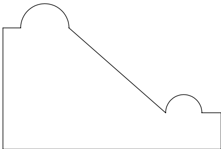
1.500" x 2.250" #5067 Panel Mold
