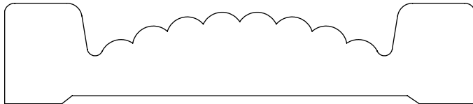
0.750" x 3.500" #2534 Casing
