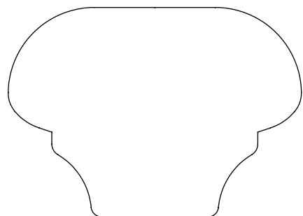
1.562" x 2.187" #6012 Hand Rail
