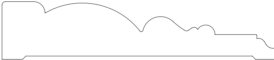
1.062" x 5.000" #2802 Casing
