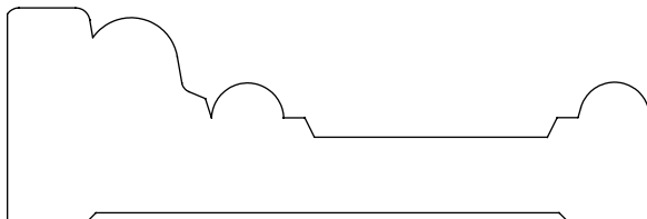
1.000" x 3.000" #2486 Casing
