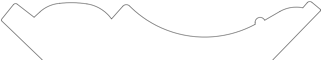
1.000" x 5.500" #4822 Crown
