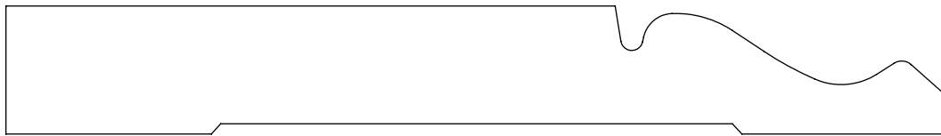
0.750" x 5.500" #1219 Base
