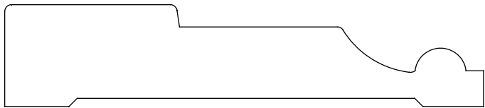
0.750" x 3.500" #2465 Casing
