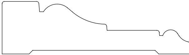
0.875" x 3.125" #2427 Casing
