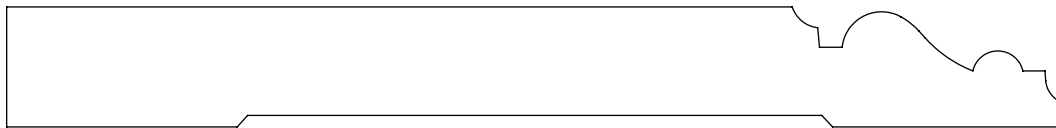
0.625" x 5.500" #1220 Base
