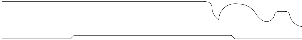
0.687" x 5.500" #1217 Base
