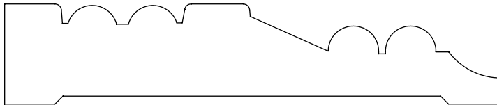
0.750" x 3.687" #2907 Casing
