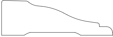
0.750" x 2.390" #2114 Casing
