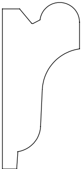
0.812" x 1.750" #4901 Crown
