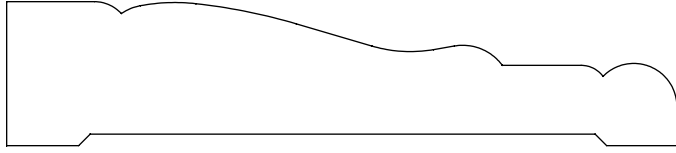
0.750" x 3.500" #2210 Casing
