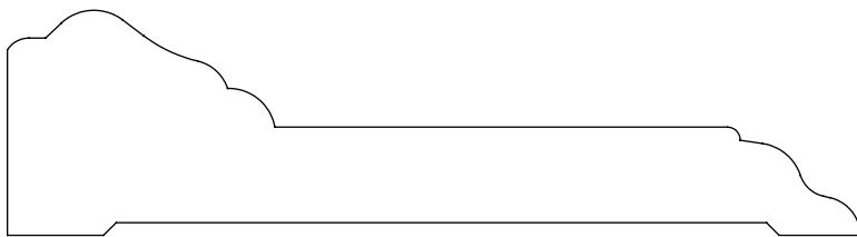
1.062" x 4.000" #2485 Casing
