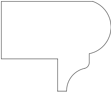
1.625" x 1.625" #6502 Nosing
