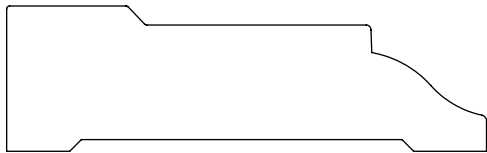
0.750" x 2.500" #2151 Casing
