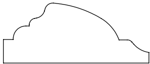
0.625" x 1.500" #5091 Panel Mold
