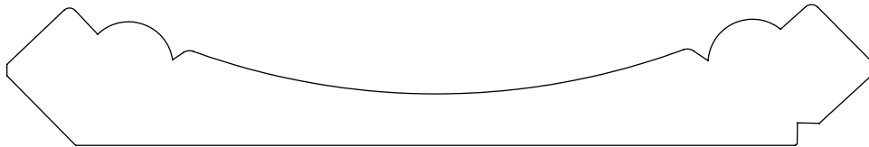
0.812" x 5.000" #4103 Crown
