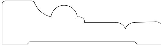
0.750" x 2.750" #2400 Casing
