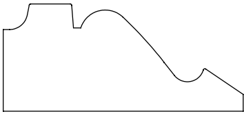
0.812" x 1.812" #5031 Panel Mold
