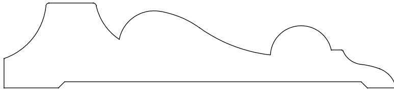
0.875" x 4.000" #2806 Casing
