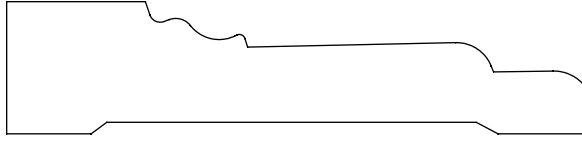
0.687" x 3.000" #2155 Casing
