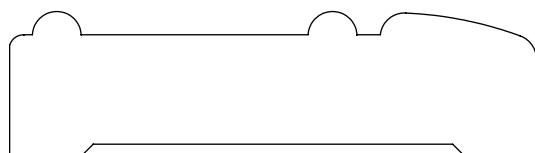
0.750" x 2.750" #8050 Chair Rail
